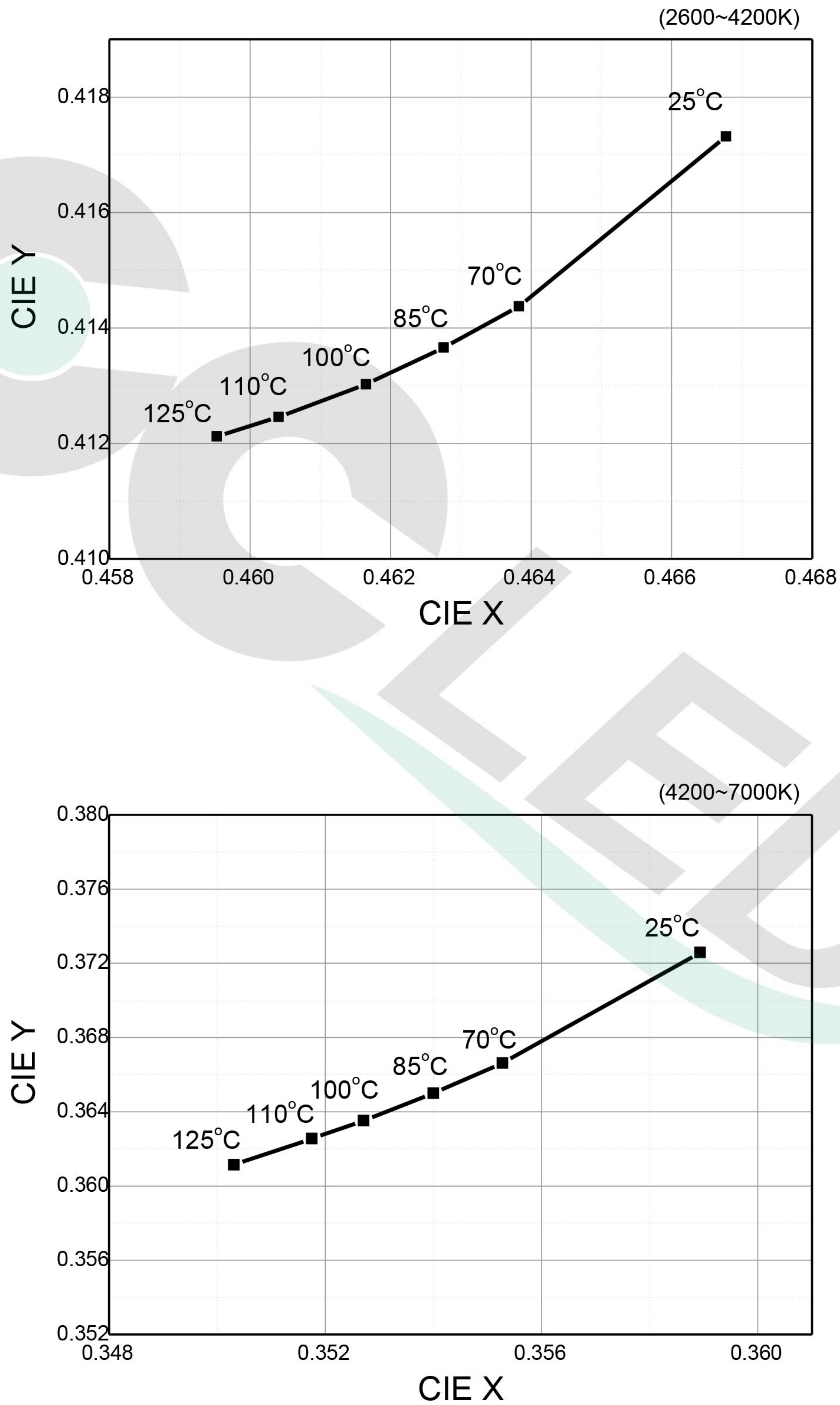
Fig 8. Chromaticity Coordinate vs. Junction Temperature, I_F=150\text{mA}
