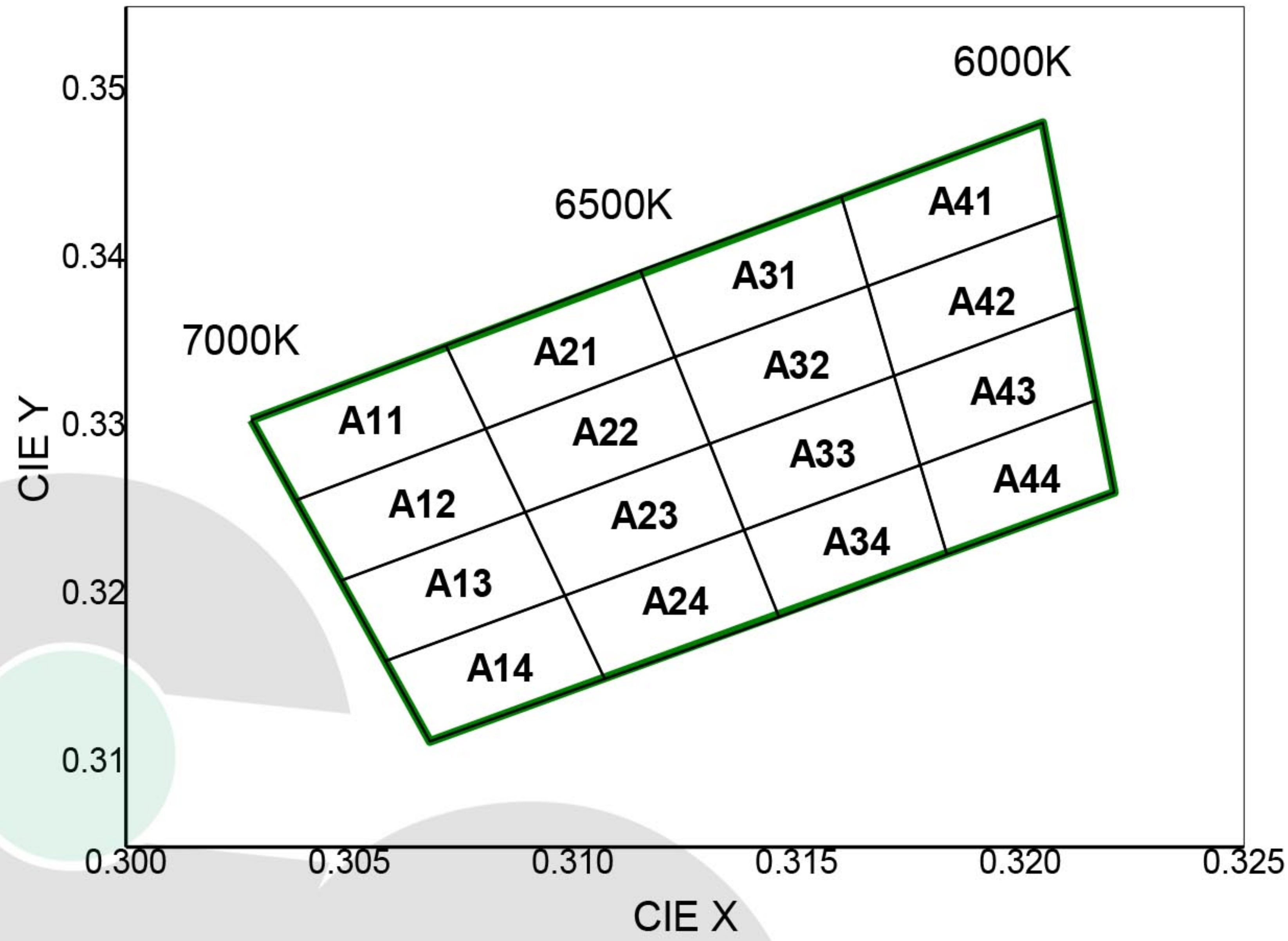
CIE Chromaticity Diagram (Cool white), T_j=25^\circ\text{C} , I_F=150\text{mA}
