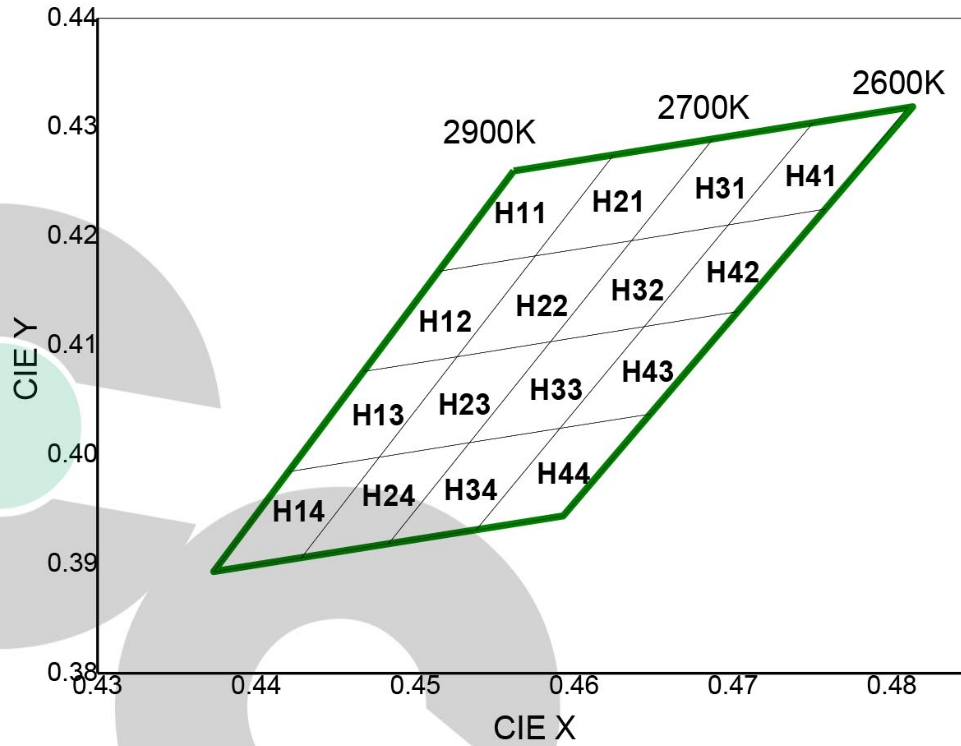
CIE Chromaticity Diagram (Warm white), T_j=25^\circ\text{C} , I_F=150\text{mA}
