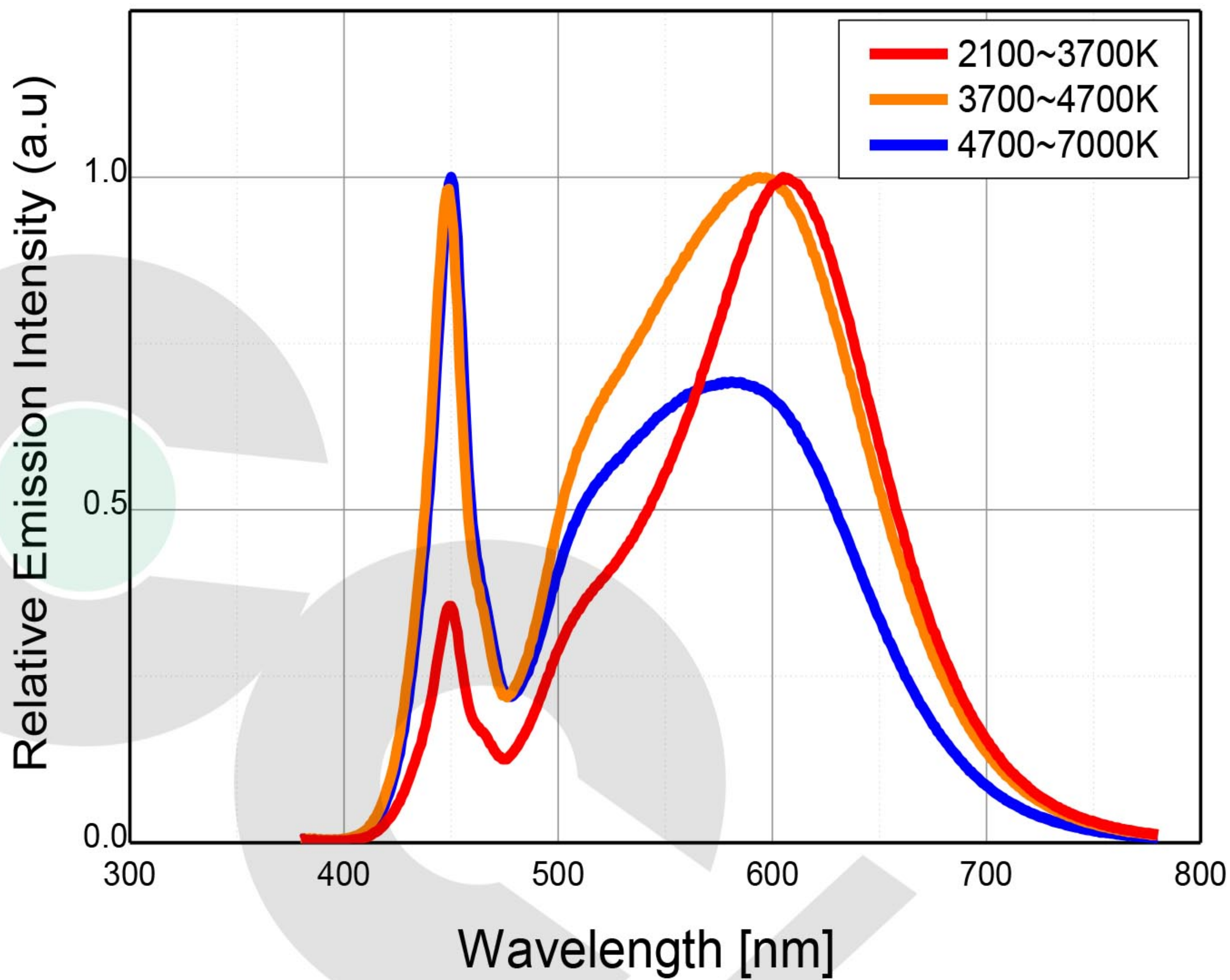
Fig 1. Color Spectrum, T_j = 25^\circ\text{C} , I_F = 150\text{mA}
