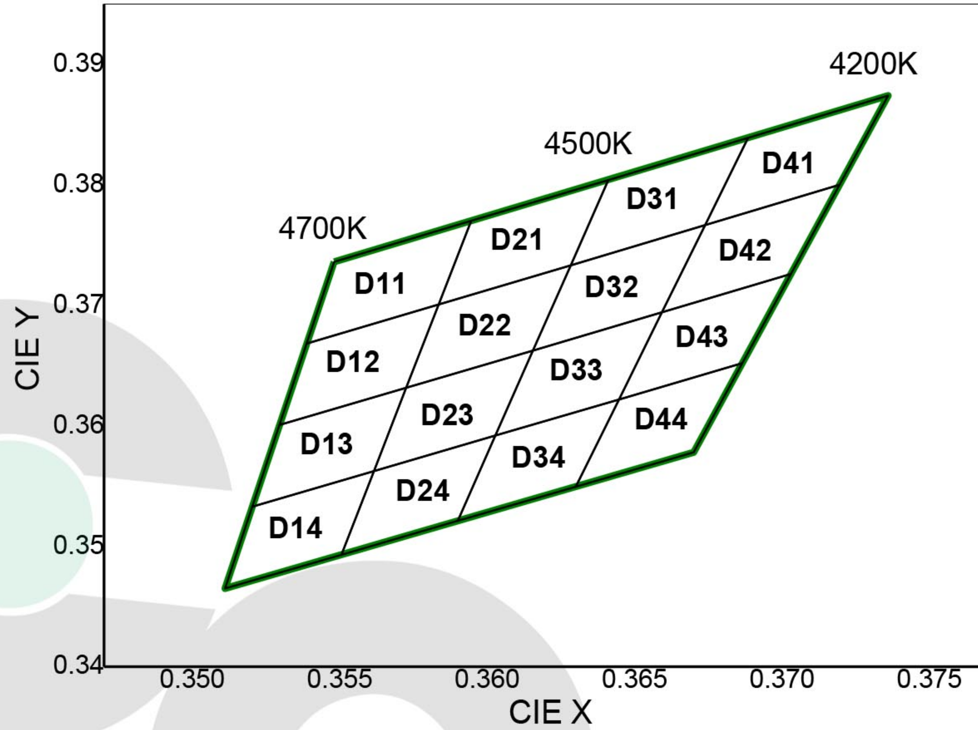
CIE Chromaticity Diagram (Neutral white), T_j=25^\circ\text{C} , I_F=150\text{mA}
