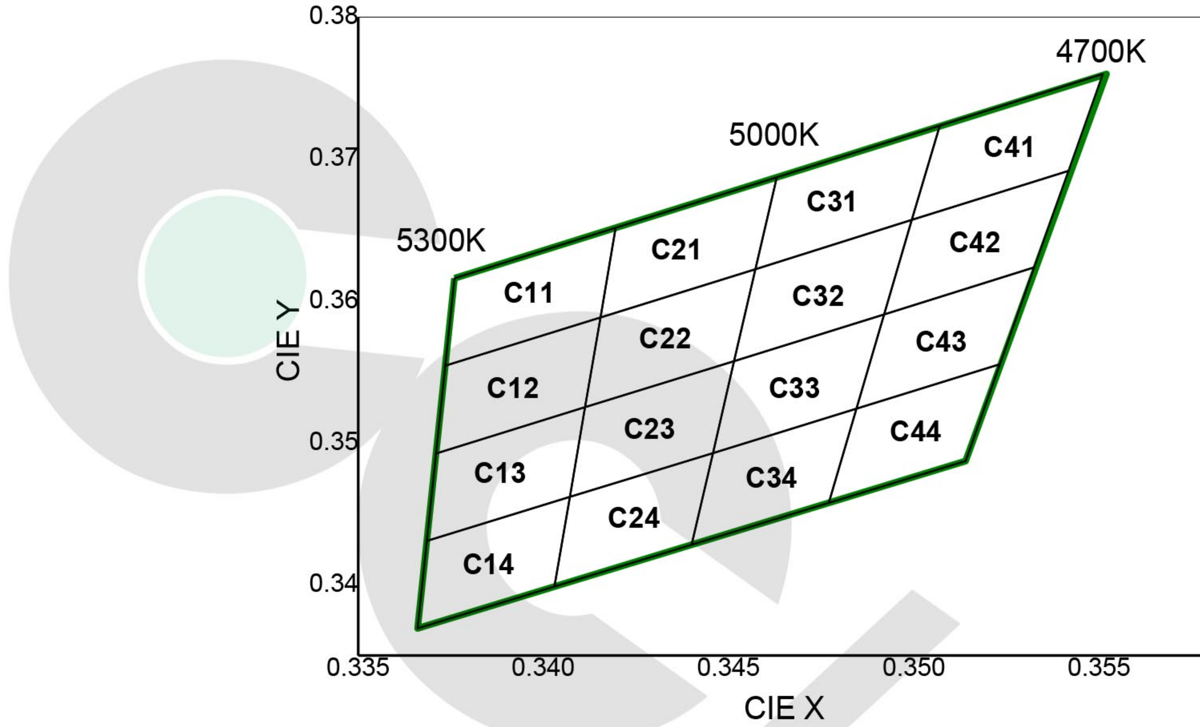
CIE Chromaticity Diagram (Cool white), T_j=25^\circ\text{C} , I_F=150\text{mA}
