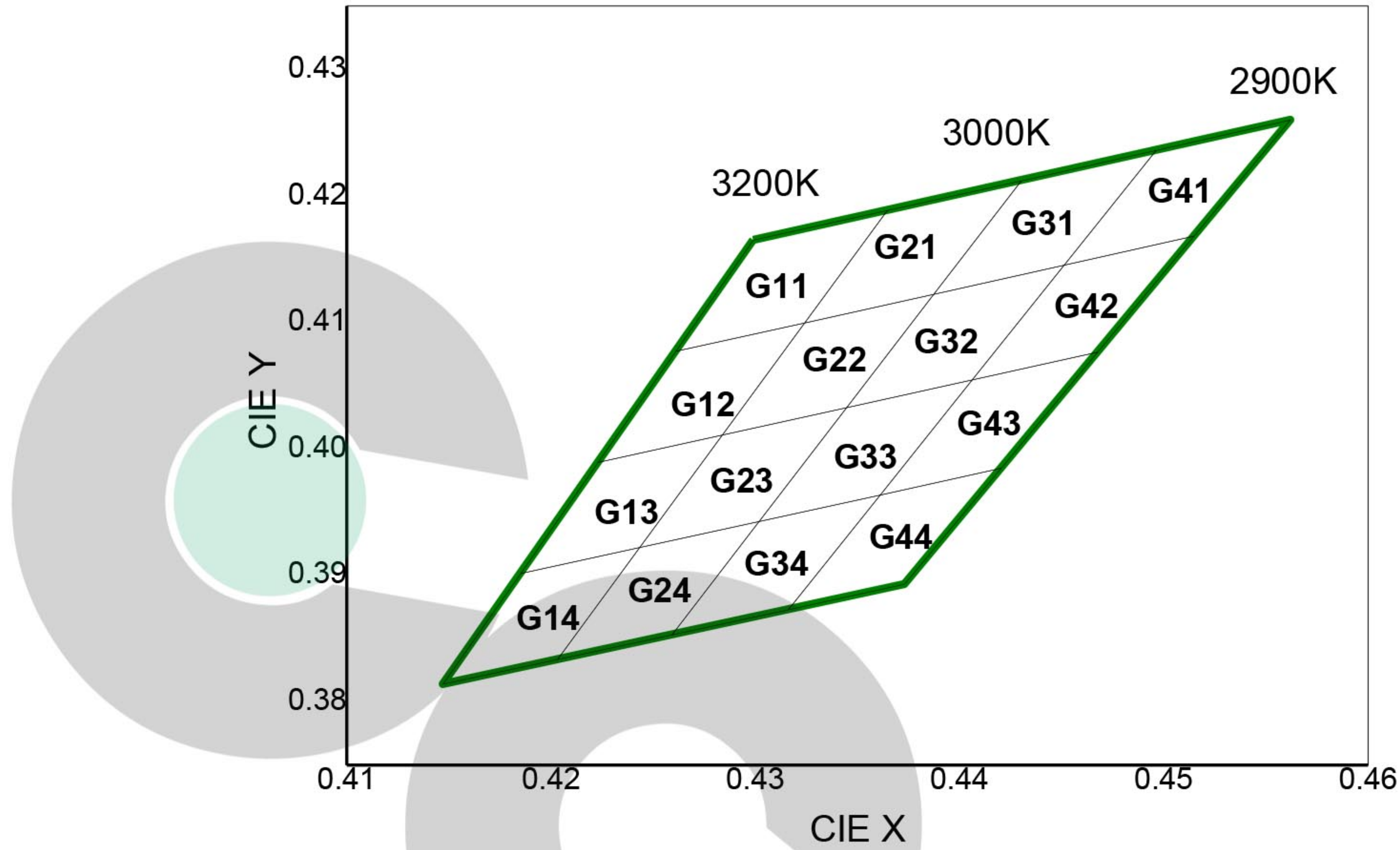
CIE Chromaticity Diagram (Warm white), T_j=25^\circ\text{C} , I_F=150\text{mA}
