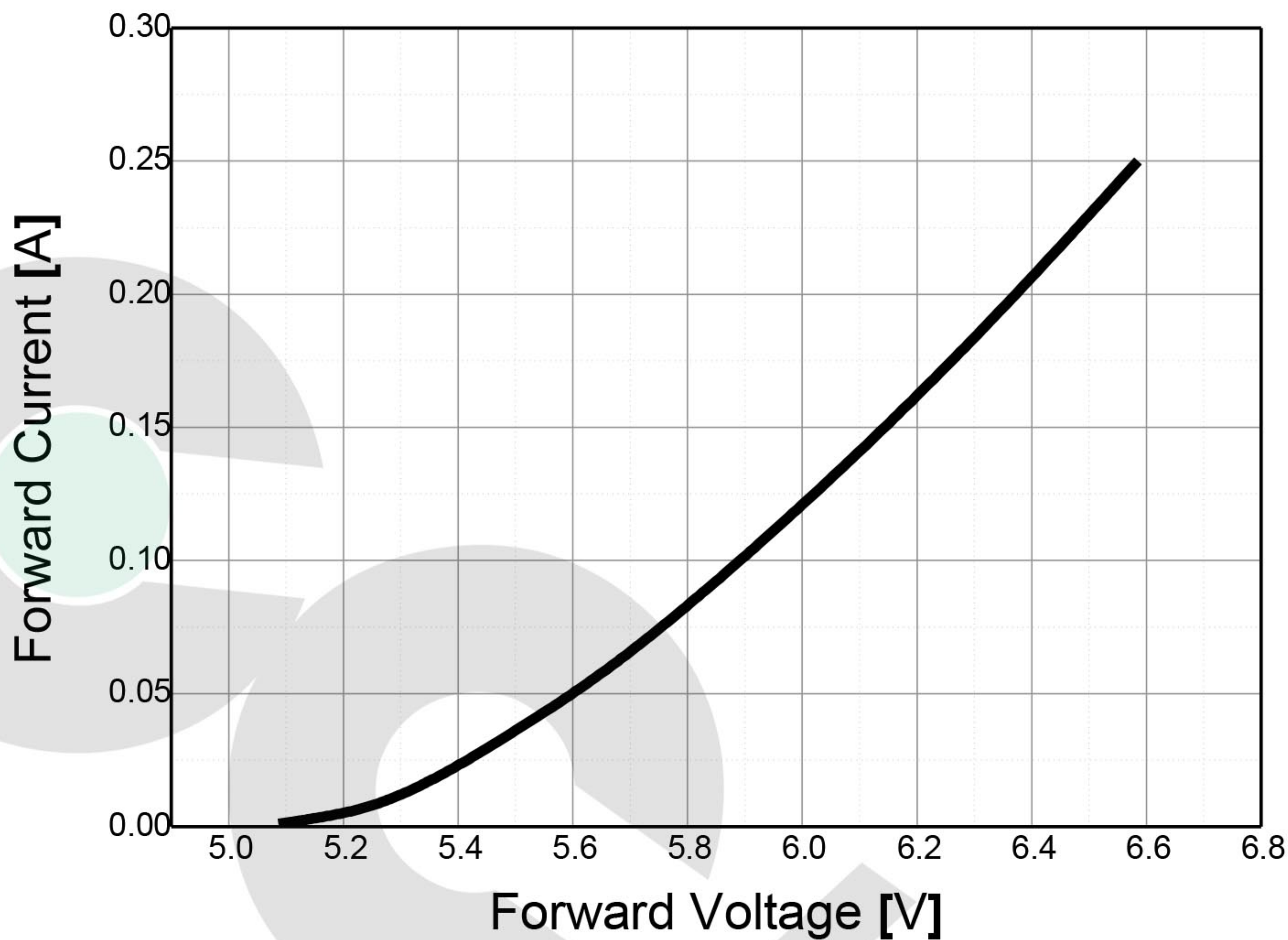
Fig 3. Forward Voltage vs. Forward Current, T_j = 25^\circ\text{C}
